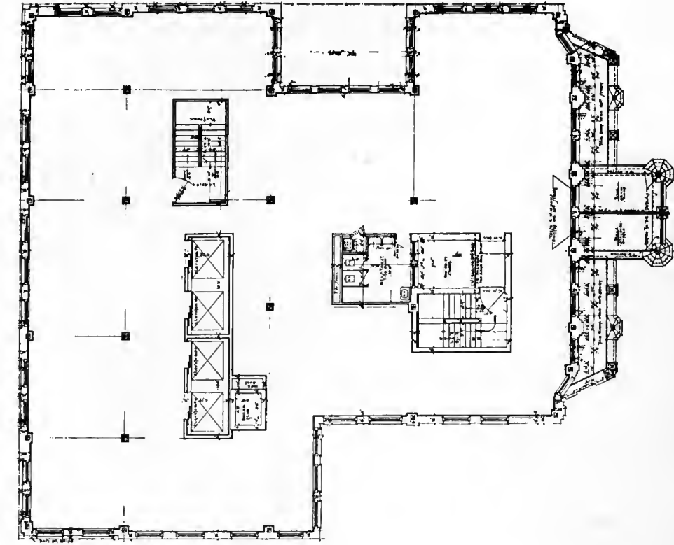
TWENTY-FIRST AND TWENTY-SECOND FLOOR PLAN
